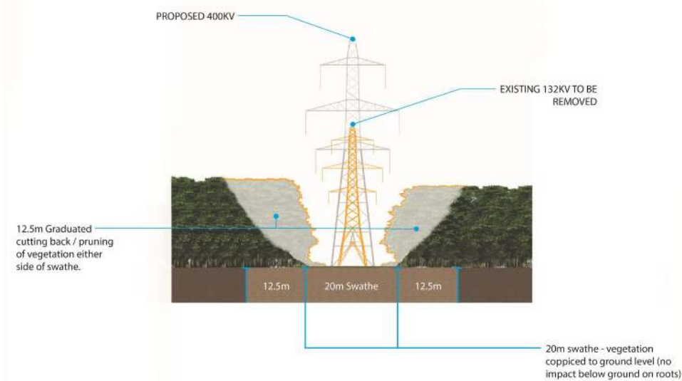
Illustration 7.1 – Sketch of 400kV Overhead Line Construction Within Woodland
